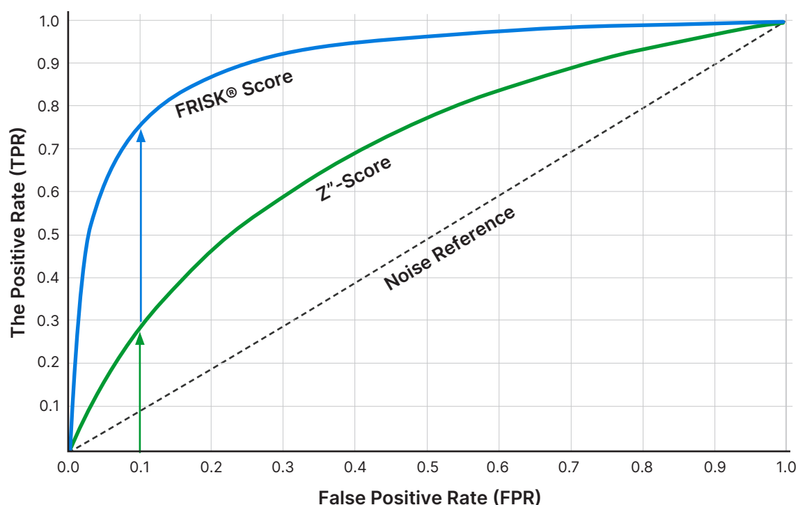
Figure 5. The ROC graph shows that the FRISK® Score can be as much as three times more effective at identifying high-risk companies than the Altman Z''-Score.
