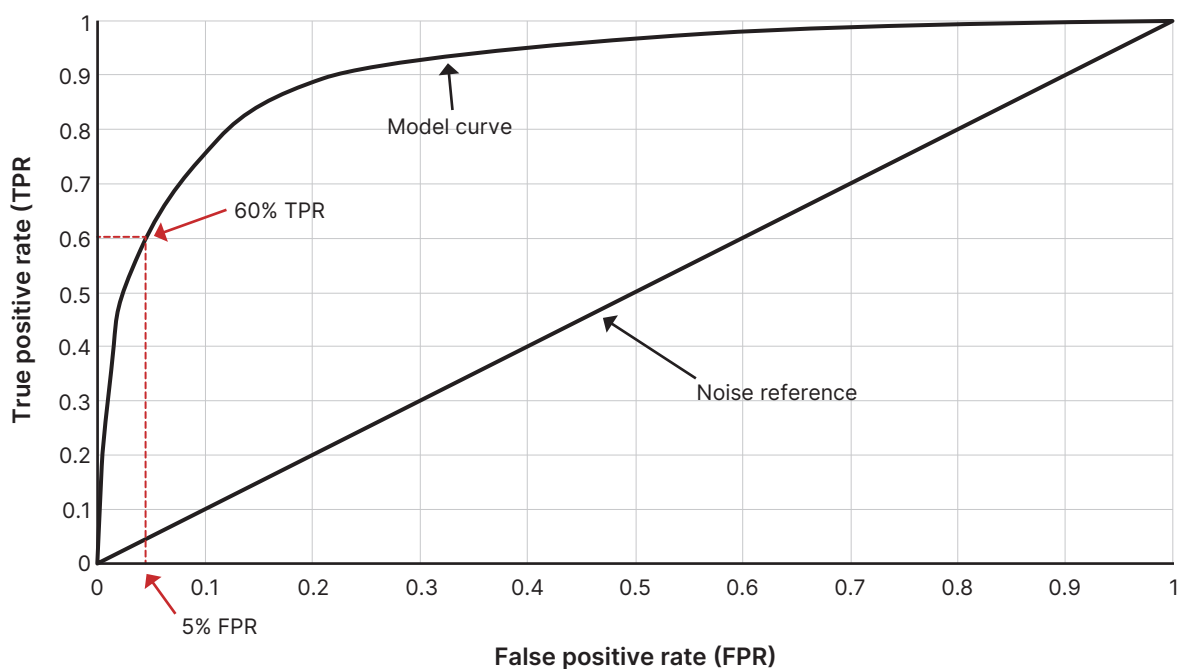
Figure 2. The ROC curve, a commonly used statistical evaluation method, shows the accuracy of the FRISK® Score. 60% of bankruptcies are identified in just the “worst 5%” of all companies scored.
