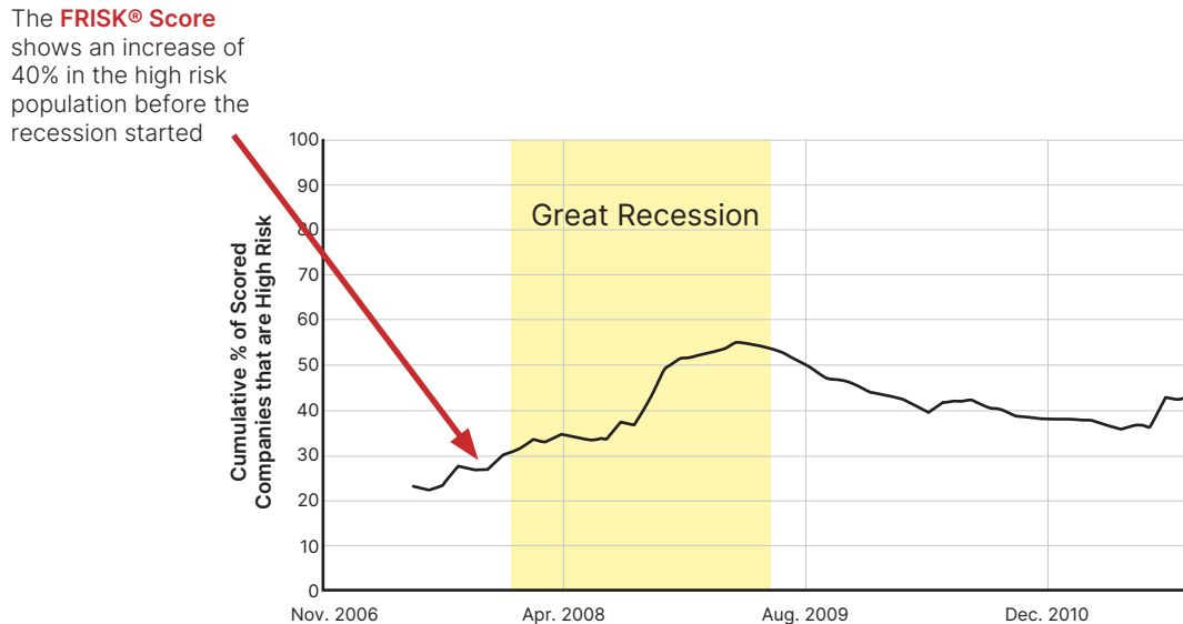
Figure 1. The FRISK® Score indicated a doubling of risky companies during the Great Recession.
