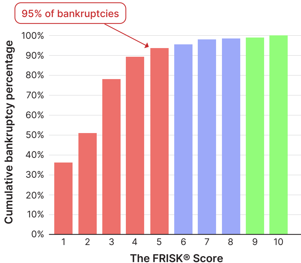
Figure 3. Showing the performance of the FRISK® Score at identifying bankruptcies occurring in the subsequent 12 months. Scores "1" to "5" (red) are high-risk, capturing 95% of bankruptcies.
